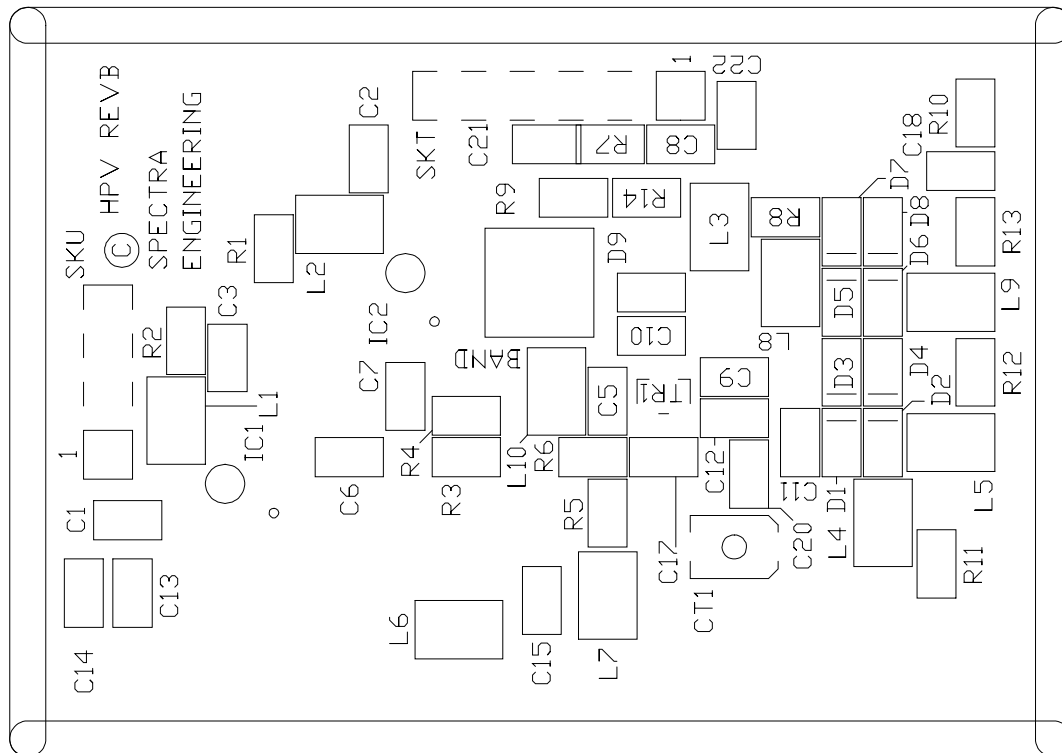
Figure 9-8 HP Rx VCO Component Overlay Bands A to Q
