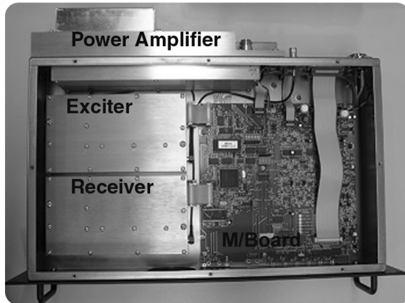
Figure 4-1 MX800 Top View
