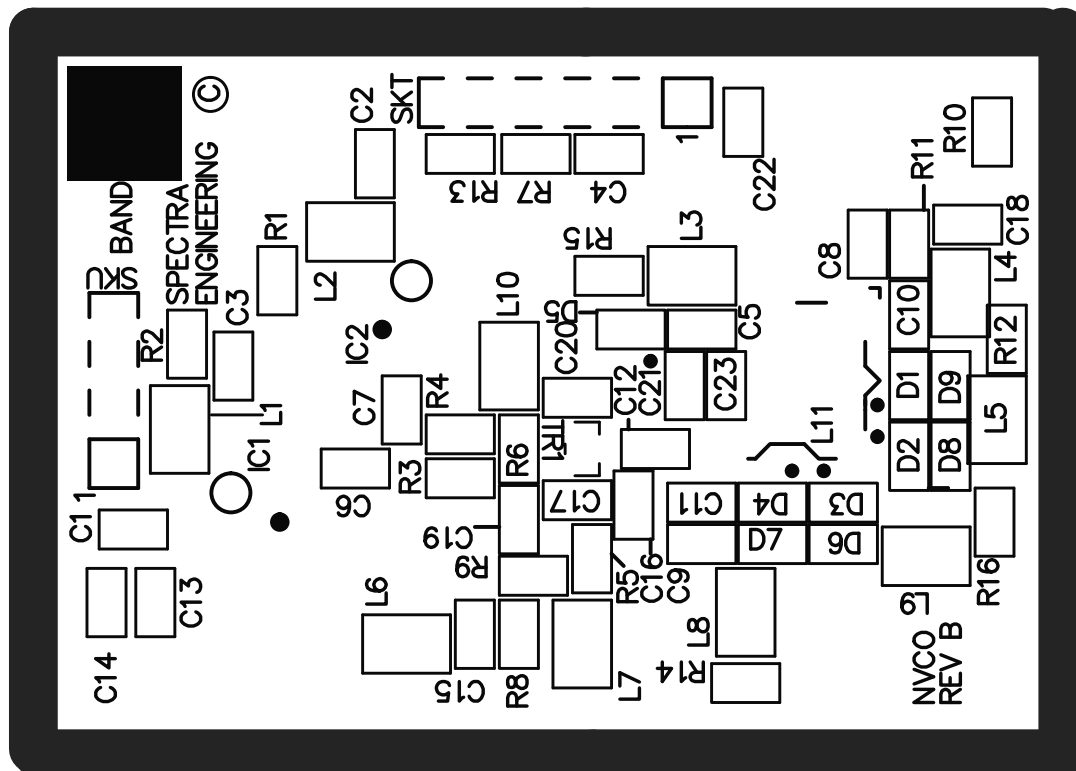
Figure 9-9 TX/RX V3 VCO Component Overlay
