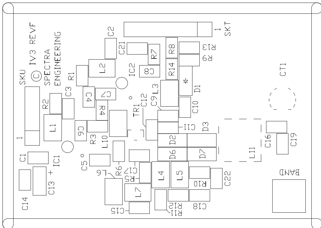
Figure 9-6 Tx and Rx VCO Component Overlay Bands A to Q3
